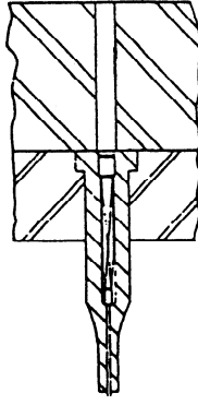
COMMON PIERCE PUNCH
