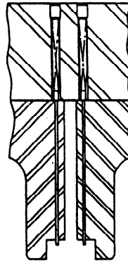
HEELED NOTCHING PUNCHES
