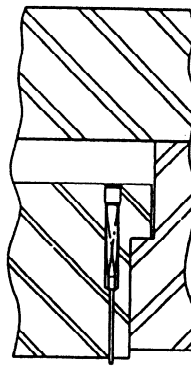
KNOCK-OUT IN COMPOUND DIE
