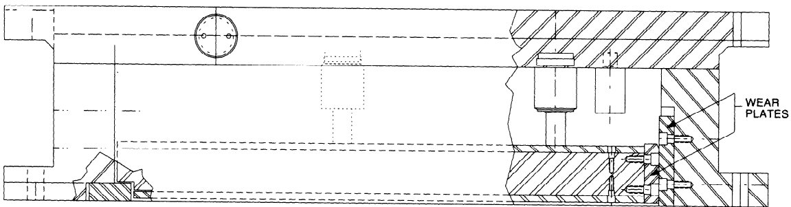
Spring Box Ram Cushion Design
