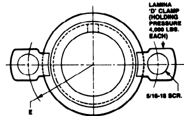
BUSHING (ASSEMBLY) (Includes bushing, clamps, screws)
