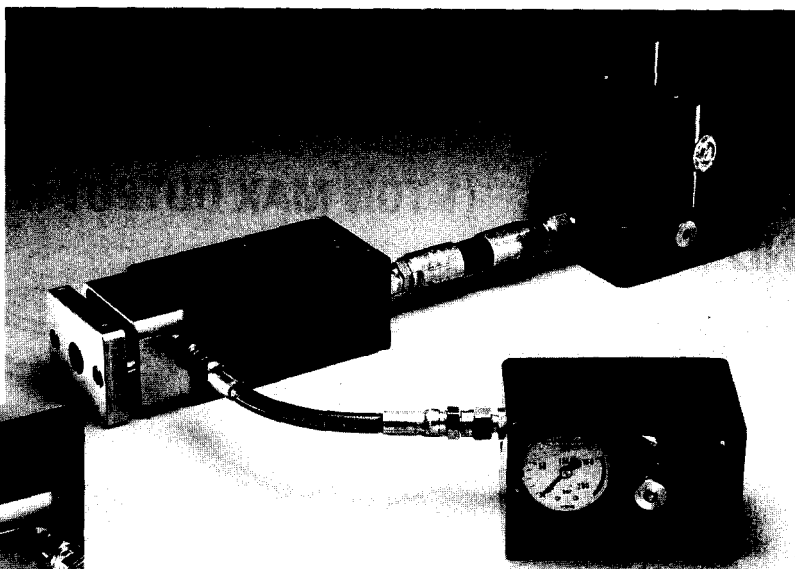
HYDROCAM™ system shown with control panel option to monitor and adjust nitrogen pressure in the H-2 piercing/forming unit.
