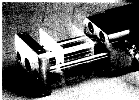
HYDROCAM™ system shown with control panel option to monitor and adjust nitrogen pressure in the H-2 piercing/forming unit.
